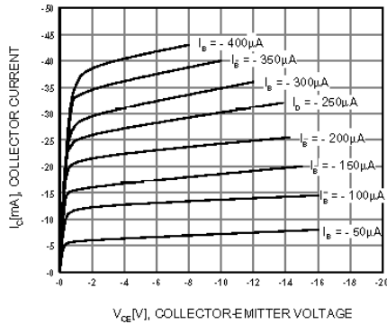
Figure 1. Static Characteristic
