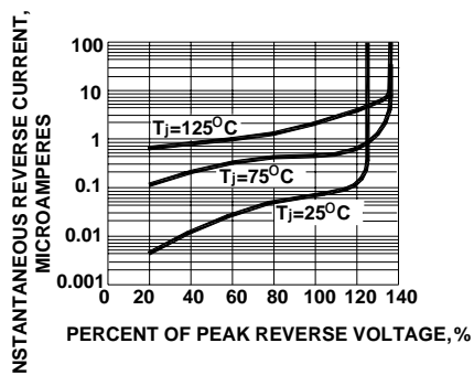
Fig. 3-TYPICAL REVERSE CHARACTERISTICS
