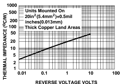
Fig. 5-TRANSIENT THERMAL IMPEDANCE
