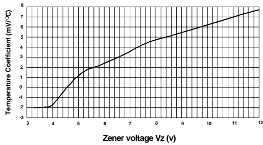
Temperature Coefficient
