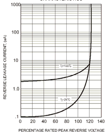
FIG.5 - TYPICAL REVERSE CHARACTERISTICS
