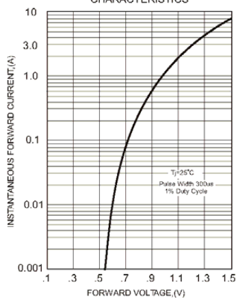
FIG.2-TYPICAL FORWARD CHARACTERISTICS
