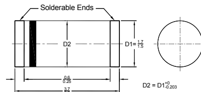
MiniMELF (DO-213AA) Plastic Package Dimensions in millimeters
