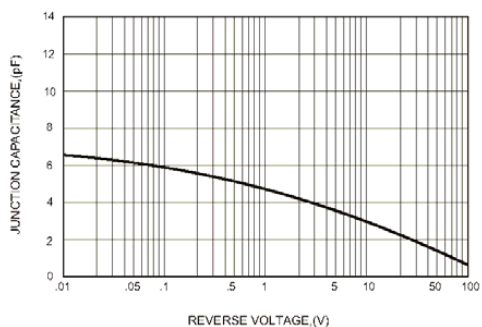
FIG.4-TYPICAL JUNCTION CAPACITANCE
