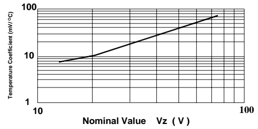
Temperature Coefficient
