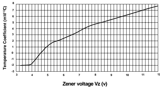
Temperature Coefficient
