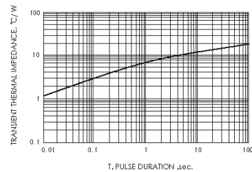
FIG.6-TYPICAL TRANSIENT THERMAL IMPEDANCE
