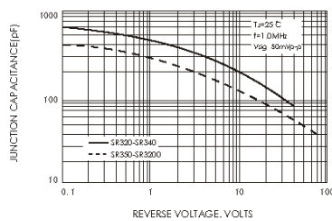
FIG.5-TYPICAL JUNCTION CAPACITANCE
