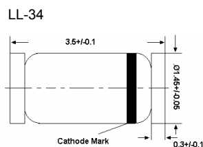
Glass case MiniMELF Dimensions in mm
