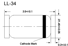
Glass case MiniMELF Dimensions in mm
