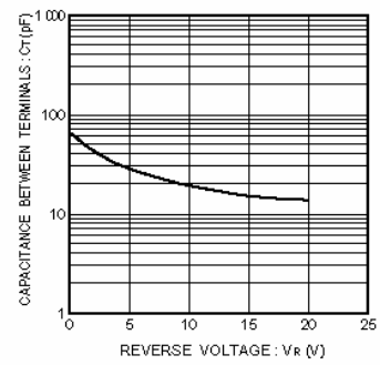
Fig. 3 Capacitance between terminals characteristic
