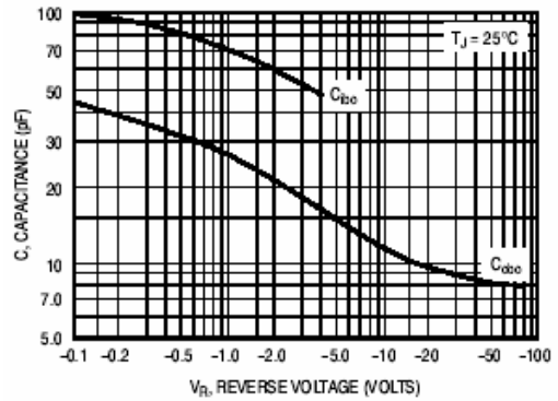
Figure 2. Capacitance
