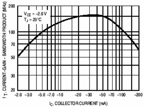
Figure 1. Current-Gain — Bandwidth Product
