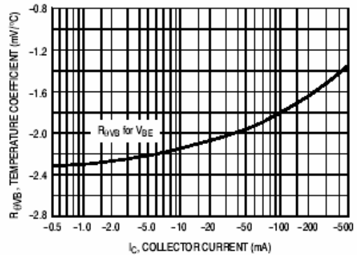
Figure 8 . Base-Emitter Temperature Coefficient
