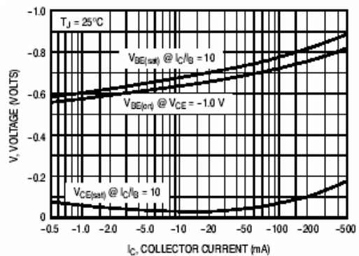
Figure 6. "ON" Voltages
