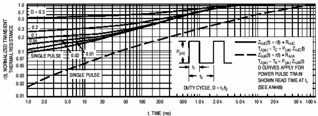
Figure 9 . Thermal Response
