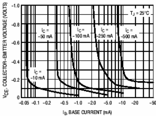
Figure 7 . Collector Saturation Region
