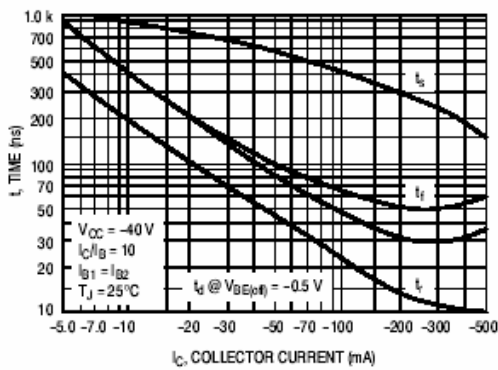
Figure 3. Switching Time
