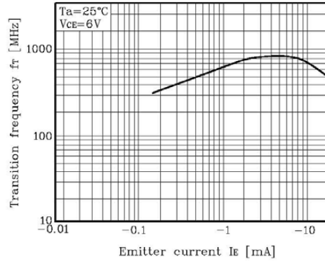
fT - IE
