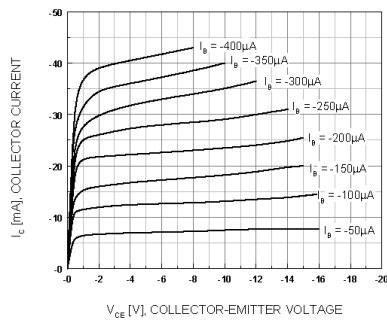
Figure 1. Static Characteristic
