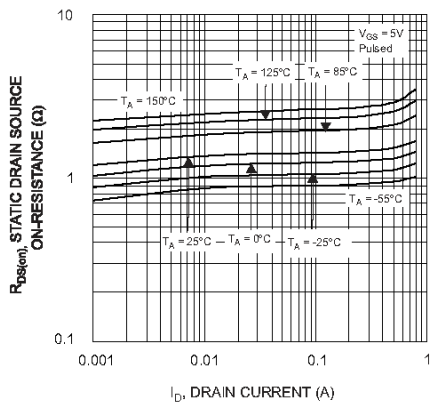
Fig. 5 Static Drain-Source On-Resistance vs. Drain Current
