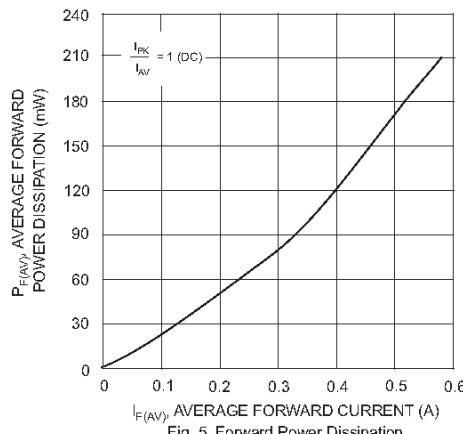
Fig. 5 Forward Power Dissipation
