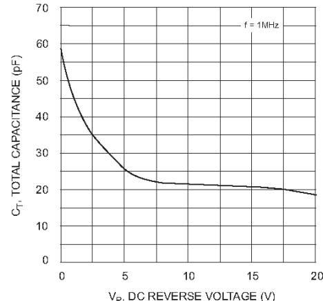
Fig. 4 Typ. Total Capacitance vs Reverse Voltage
