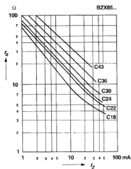
Dynamic resistance versus Zener current
