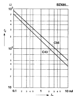
Dynamic resistance versus Zener current
