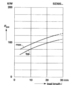
Thermal resistance versus lead length
