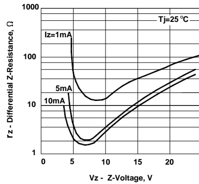
Differential Z-Resistance vs. Z-Voltage
