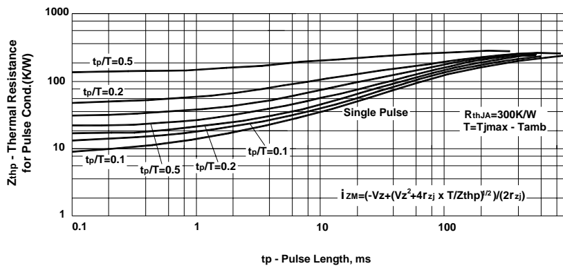
Thermal Response
