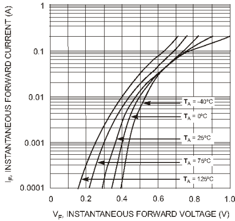
Fig. 1 Typical Forward Voltage
