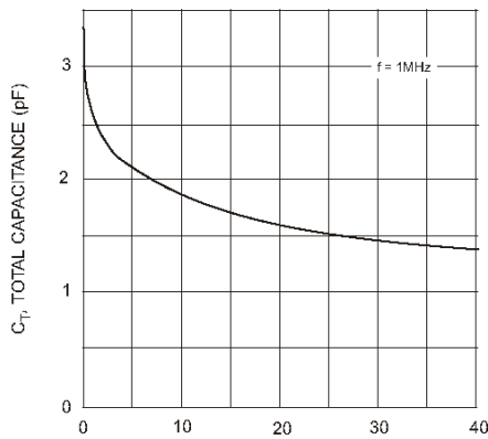
Fig. 3 Typical Capacitance
