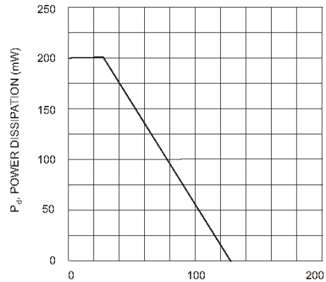
Fig. 4 Power Derating Curve, Total Package
