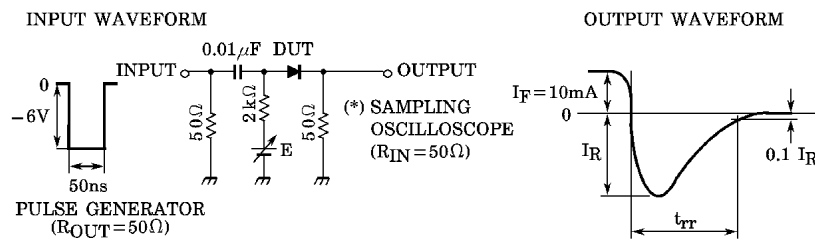
Fig.1 Reverse recovery time ( t_{rr} ) test circuit
