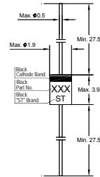
Glass Case DO-35 Dimensions in mm
