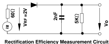
Rectification Efficiency Measurement Circuit
