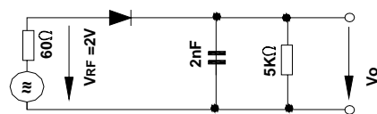
Rectification Efficiency Measurement Circuit
