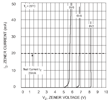
Fig. 4 Zener Breakdown Characteristics
