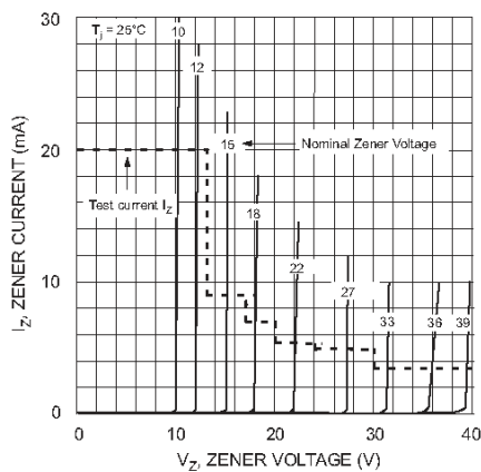
Fig. 5 Zener Breakdown Characteristics
