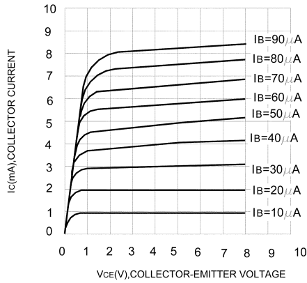
STATIC CHARACTERISTIC
