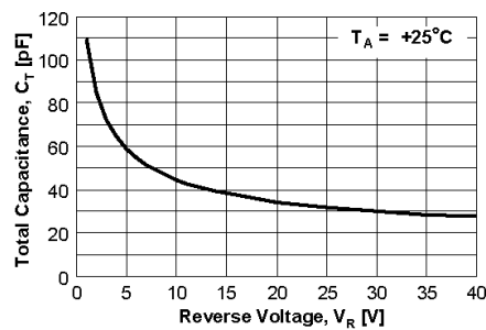
Figure 3. Total Capacitance
