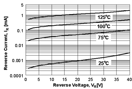
Figure 2. Reverse Current vs Reverse Voltage
