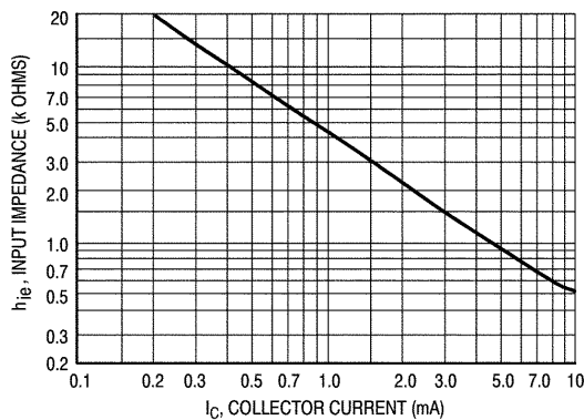
Figure 11. Input Impedance
