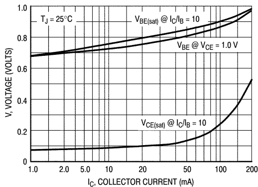
Figure 15. "ON" Voltages
