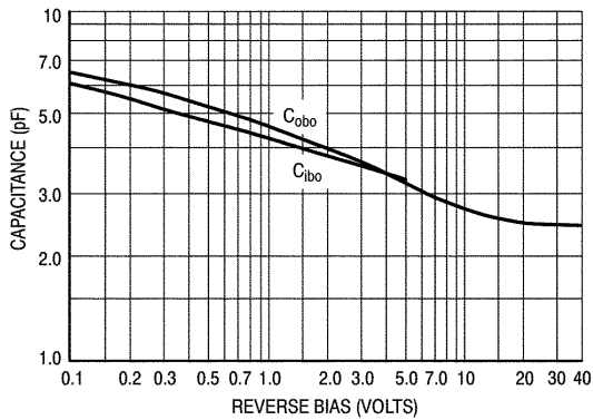
Figure 3. Capacitance
