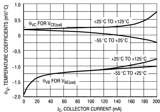
Figure 16. Temperature Coefficients
