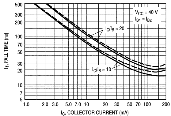
Figure 6. Fall Time
