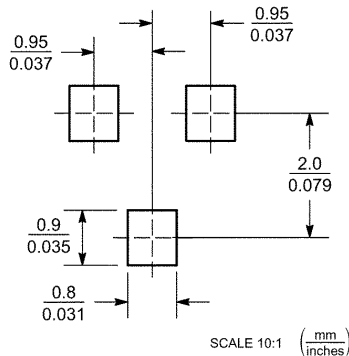
Figure 17. SOT-23
