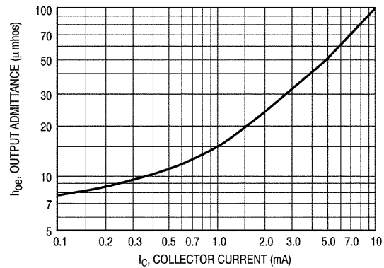
Figure 10. Output Admittance
