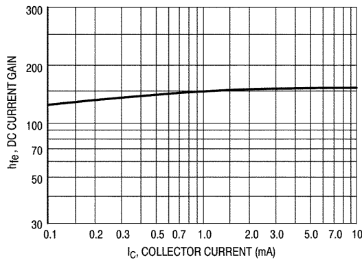
Figure 9. Current Gain
