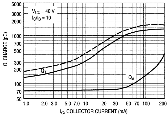
Figure 4. Charge Data
