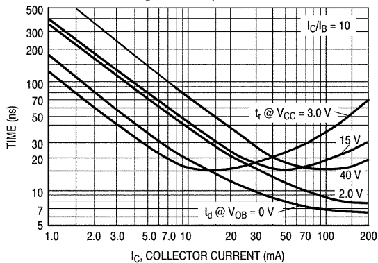
Figure 5. Turn-On Time
