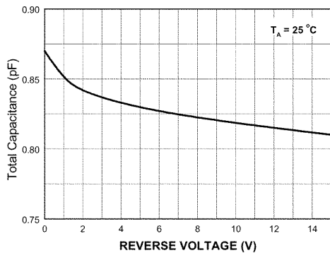
Figure 7. Total Capacitance
