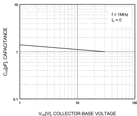
Figure 4. Output Capacitance
