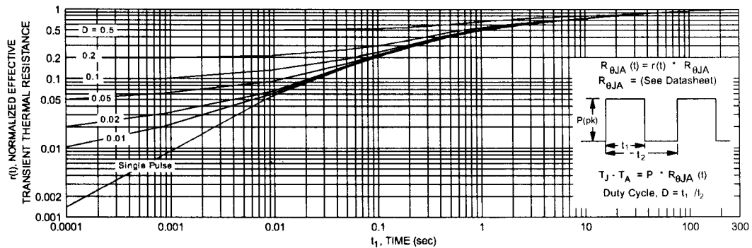
Figure 17. SOT-23, 2N7002 / NDS7000A Transient Thermal Response Curve
