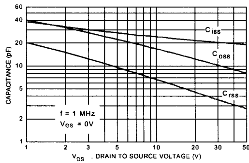
Figure 9. Capacitance Characteristics
