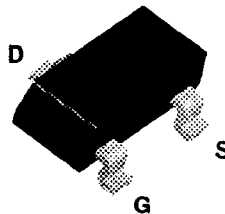
SOT-23 (TO-236AB) 2N7002/NDS7002A
