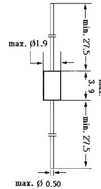
Glass case JEDEC DO-35 Dimensions in mm
