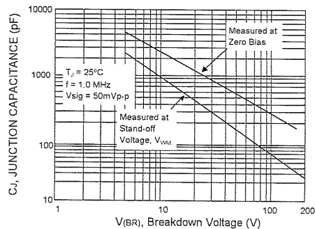
FIG.6 - TYPICAL JUNCTION CAPACITANCE UNI-DIRECTIONAL
