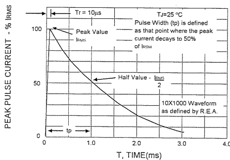
FIG.5 - PULSE WAVEFORM
