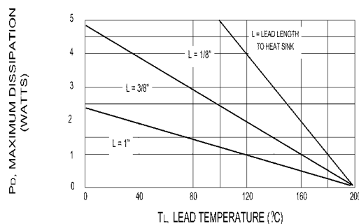
Fig. 1 Power Temperature Derating Curve
